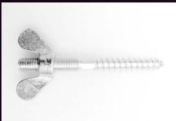
Standard mounting building installation, 90° wall bracket, wedge bolt and wing nut, M8 x 80
